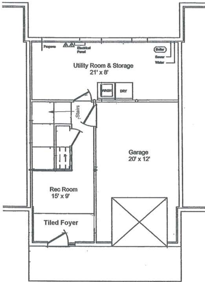
Unit 92 B- Lower Level Plan
